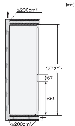
KFN7733F, KFN7733E, side view
