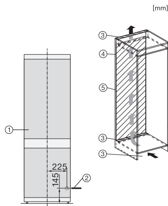
KFN7733F, KFN7733E, installation
